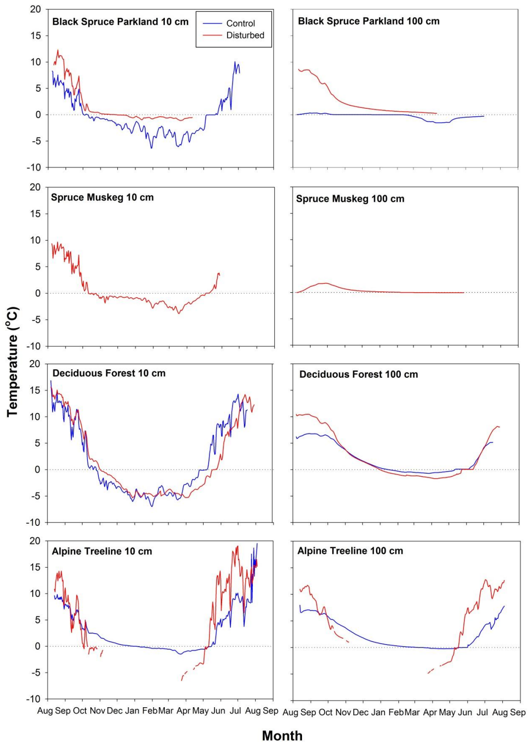
Figure 3-8: Near-surface ground temperatures recorded at 10cm and 100cm below the ground surface from August 2012 to August 2013 at disturbed (red) and undisturbed (blue) sites in black spruce parkland, spruce muskeg, deciduous forest, and alpine treeline terrain types. Lines show the daily mean temperatures (°C). The dashed reference line shows 0°C.
