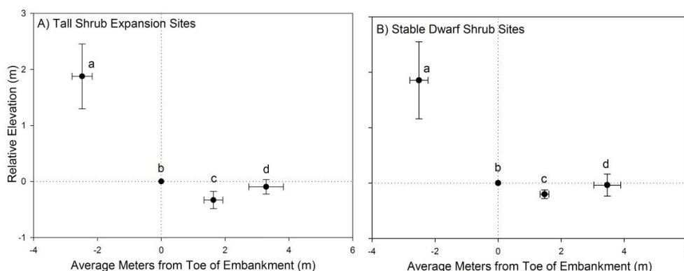
Figure 2-8: Relative elevation of the highway embankment and adjacent terrain obtained from total station surveys at A) tall shrub expansion and B) stable dwarf shrub sites. Each plot shows the average x (meters from toe of embankment) and y (relative elevation in meters) position of the highway embankment at 4 points: (a) embankment shoulder, (b) toe of the embankment, (c) minimum elevation adjacent to the embankment, and (d) first point away from the road where the ground begins to level. Error pars indicate the 95% confidence interval of the mean height of these points. Dashed lines show the position (x and y) of the embankment.
