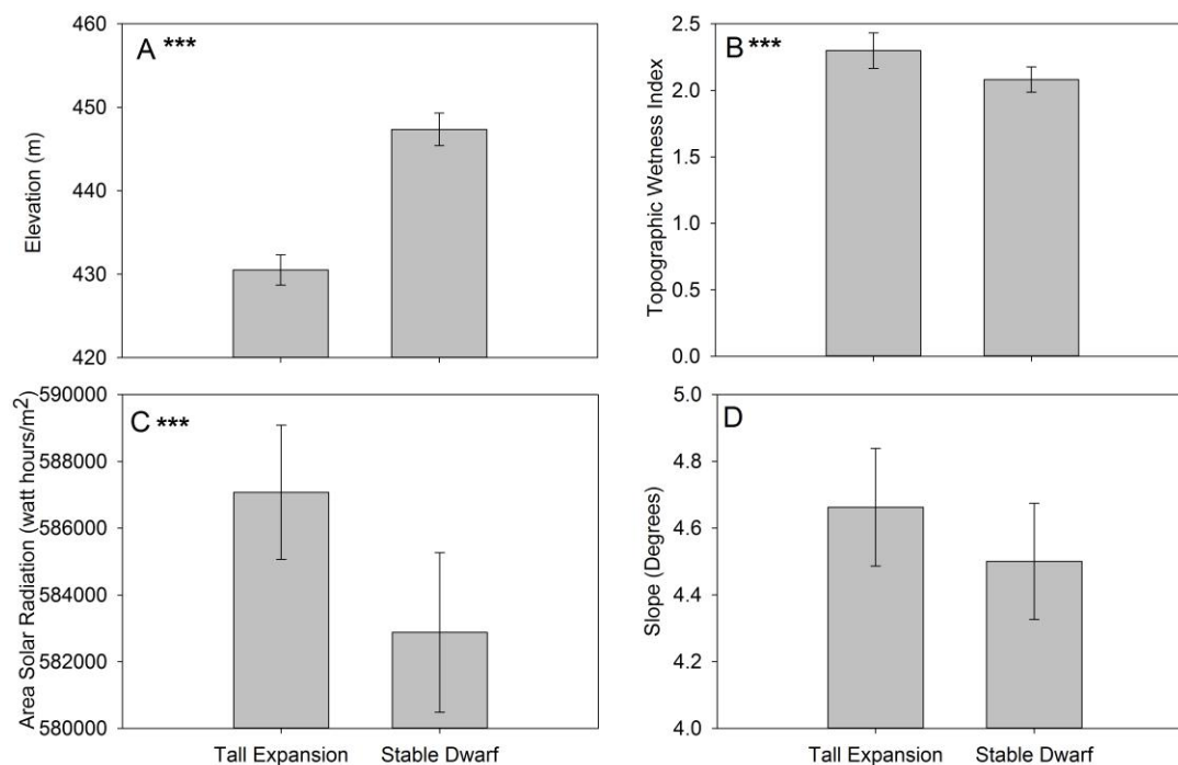
Figure 2-7: Abiotic response variables derived from GIS for stable dwarf shrub sites (Stable Dwarf) and tall shrub expansion sites (Tall Expansion) adjacent to the Dempster Highway: (A) Average elevation (m), (B) Average topographic wetness index (unitless), (C) Average untransformed area solar radiation (watt hours per m 2 ), (D) Average slope (degrees). Bars show the mean of 1000 random points for each site type. Error bars illustrate the 95% confidence interval of the mean. Three asterisks (***) indicate that the contrast is significantly different ( \alpha=0.05 ).
