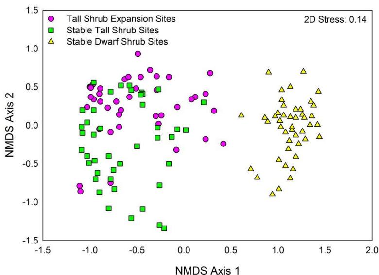
Figure 2-4: Non-metric multidimensional scaling (NMDS) ordination of plant community composition based on a Bray-Curtis similarity matrix. Symbols represent subplots sampled in 3 site types adjacent to the Dempster highway.
